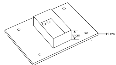
Back View Dimension
